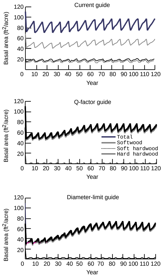
Figure 6—Basal area of loblolly pine stand by management regime (site 2).
