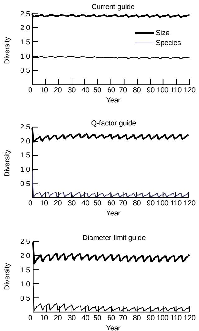
Figure 7—Diversity of loblolly pine stand by management regime (site 2).
