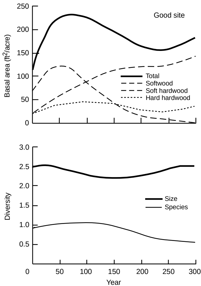
Figure 4—Basal area and diversity (Shannon's index) of undisturbed loblolly pine stand on good site (site 2).
