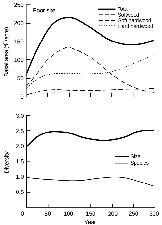
Figure 5—Basal area and diversity (Shannon's index) of undisturbed loblolly pine stand on poor site (site 6).
